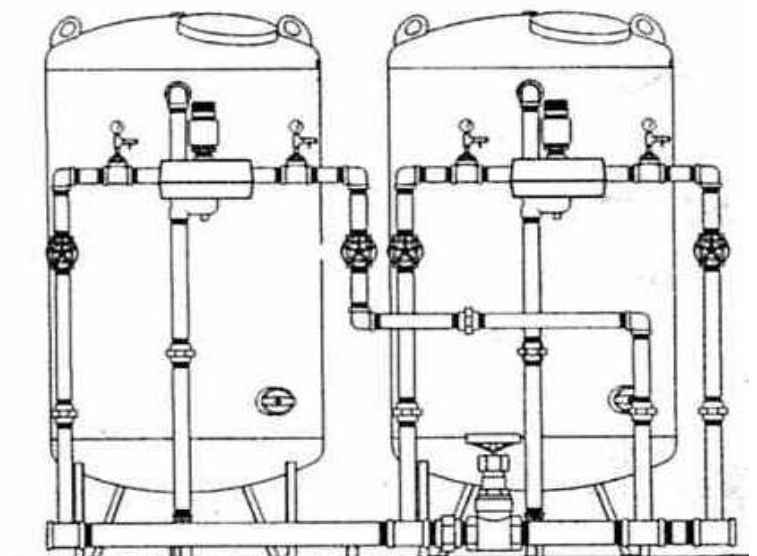
Steel Filters with Automated Valves
